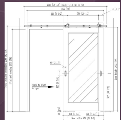
TECH DRAWING
