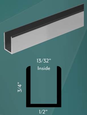
Fixed panel U channel Model ZSS-4104
