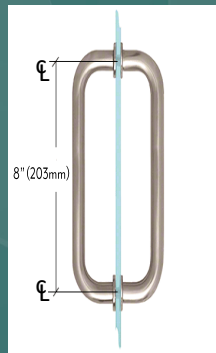
8" x 8" back-to-back pulls
