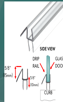
Door sweep with drip rail
