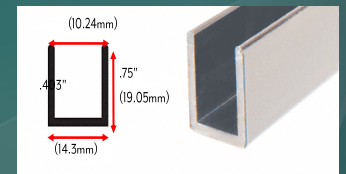
Fixed panel U channel
